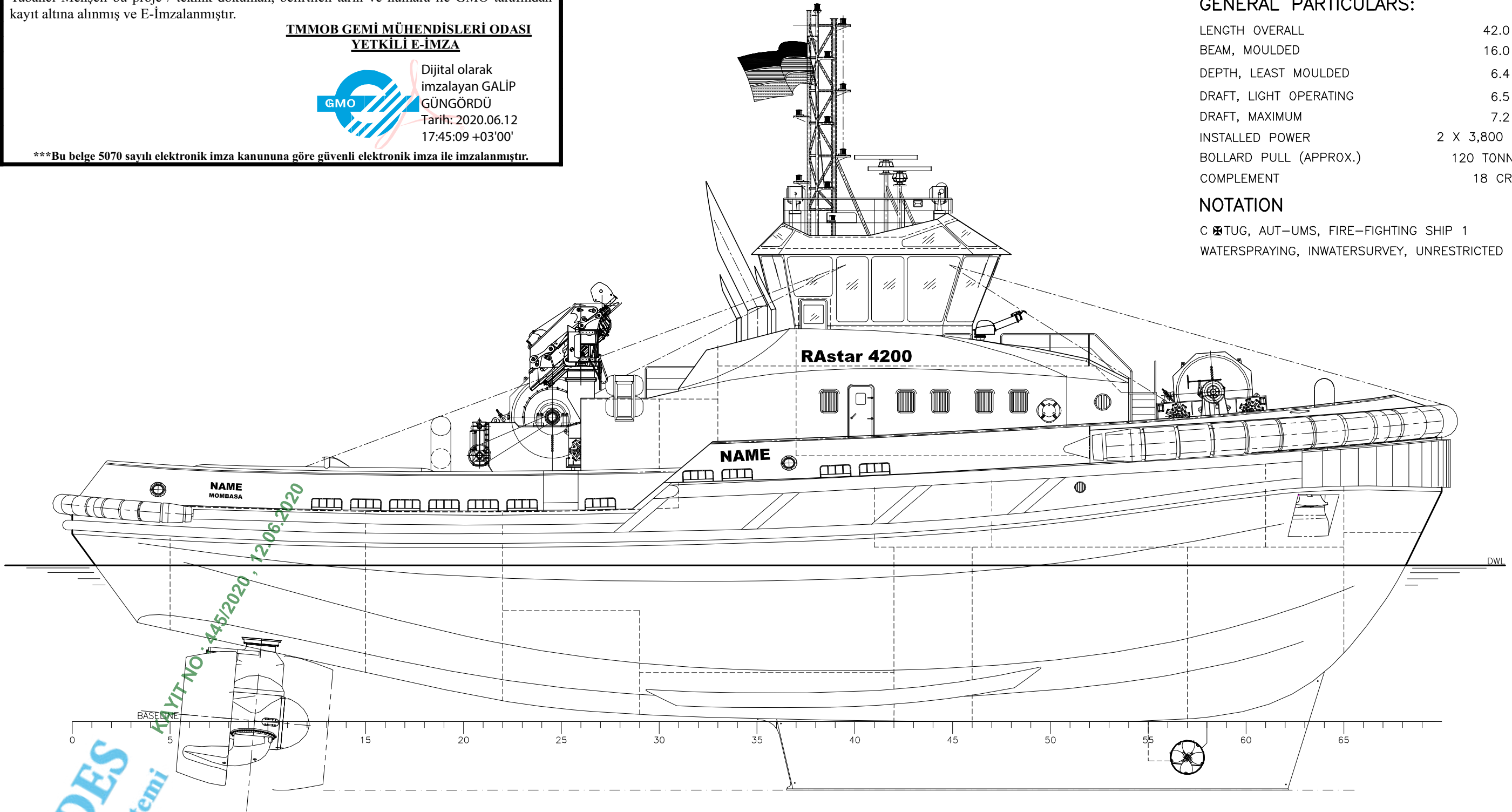
OUTBOARD PROFILE
